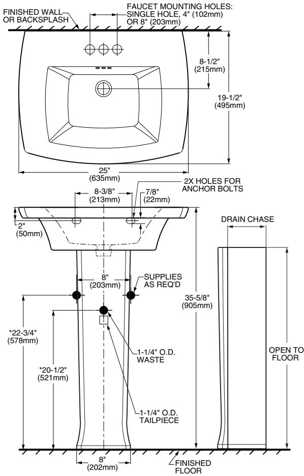
PEDESTAL CONFIGURATIONS
