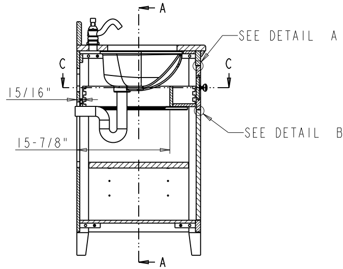
SECTION B-B SCALE 3:50
