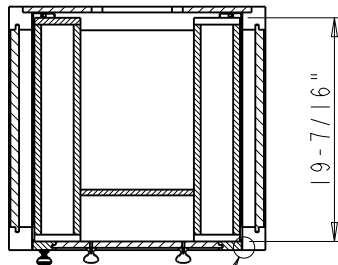
SEE DETAIL C SECTION C-C
