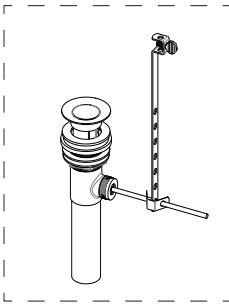
Drain Assembly
