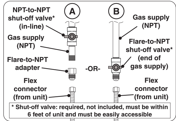
Fig. 20-1 Connecting to a gas line
