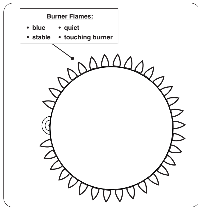
Fig. 35-1 Proper flame appearance
