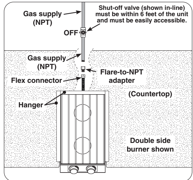
Fig. 20-2 Household LP & natural gas diagram
