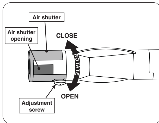
Fig. 35-2 Side burner air shutter adjustment detail
