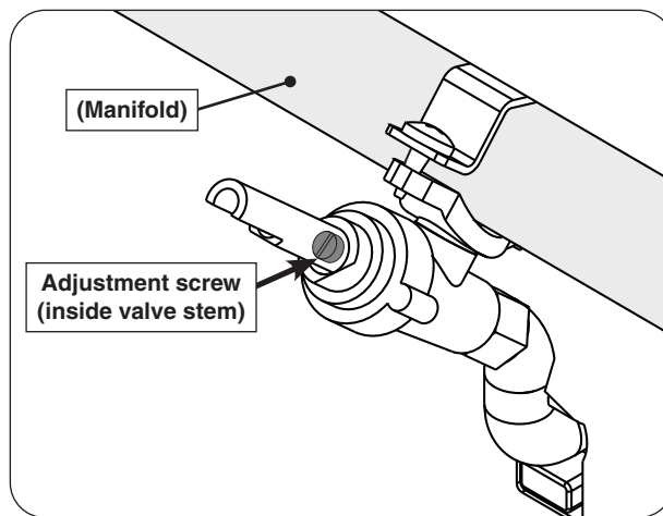
Fig. 36-3 Valve adjustment screw location
