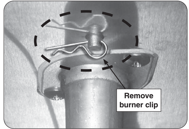
Fig. 32-1 Remove burner clip
