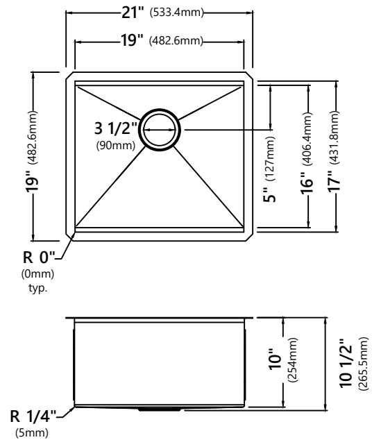
Model #: KWU111-21 Sink Dimensions: 21" x 19" x 10" Min Cabinet Size: 24"
