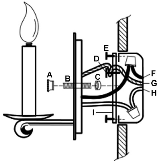
This illustration represents a typical fixture and may not match every style.
