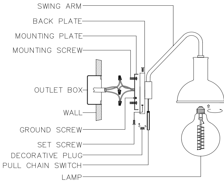
HARDWIRING TO OUTLET
